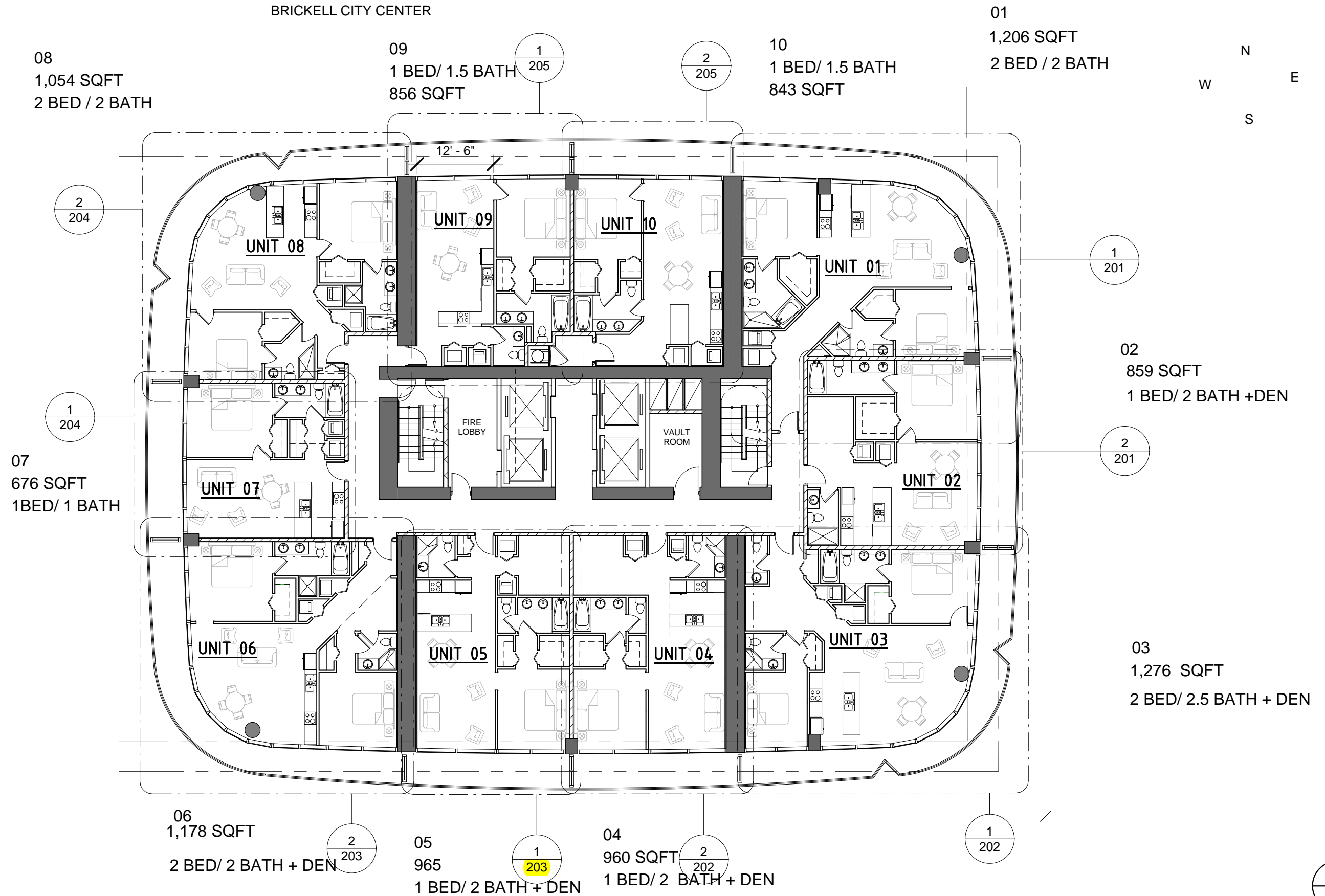
1 EAST TOWER-1ST LEVEL FLOOR PLAN 1/16" = 1'-0"
